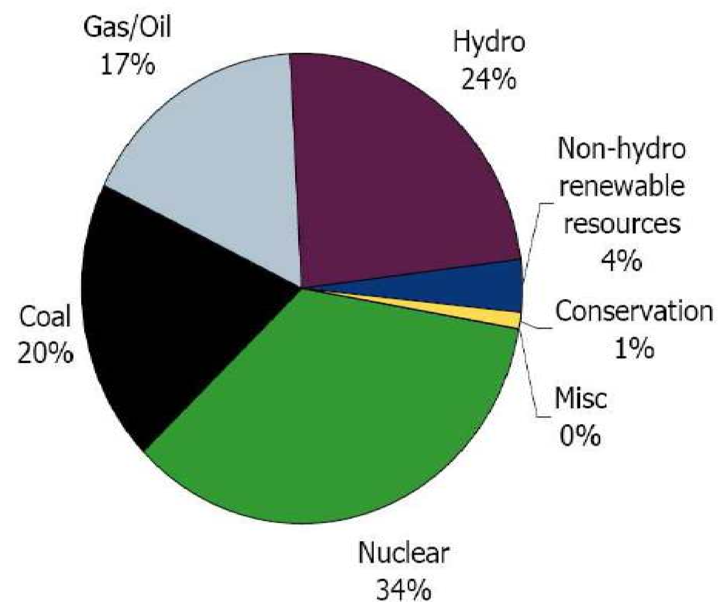
Installed Generation and Conservation 2007
